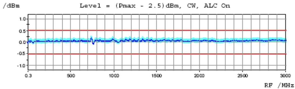
Measured level vs. frequency at 0.0 dBm
